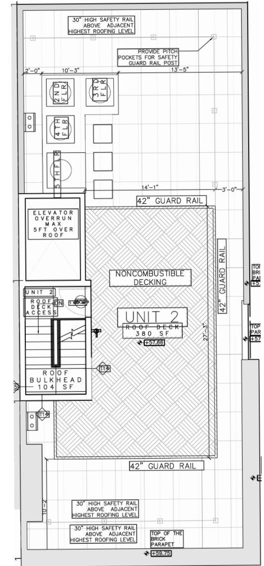
ROOF DECK
